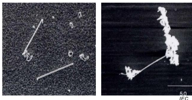
Figure B.3 – Trichite filamentaire
