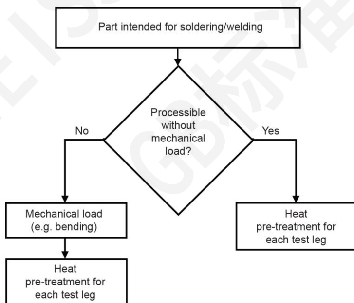
Figure 3 – Flow for treatment and/or bending and heat treatment
