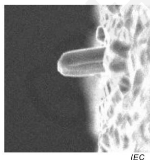
Figure B.2 – Trichite colonnaire
