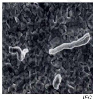
Figure B.5 – Trichite en spirale
