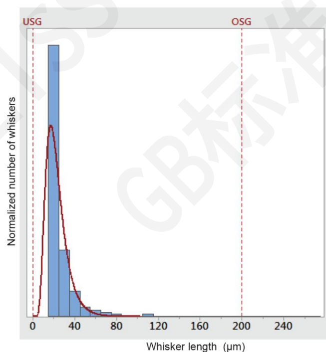
Figure C.2 – Histogram of whisker lengths and fitted log-normal distribution
