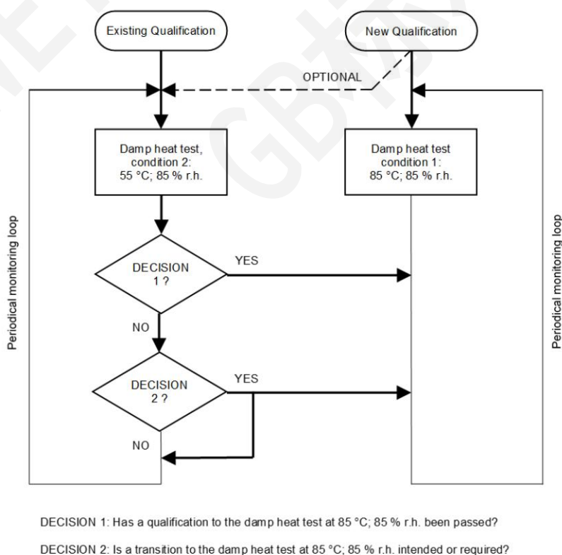
Figure E.1 –Transition paths for damp-heat testing of components
