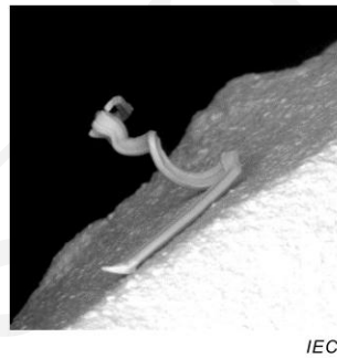
Figure B.4 – Kinked whisker
