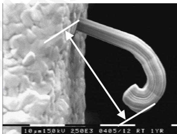
Figure A.2 – Example for whisker length measurement
