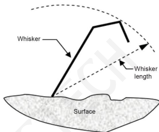
Figure A.1 – Estimation of whisker length
