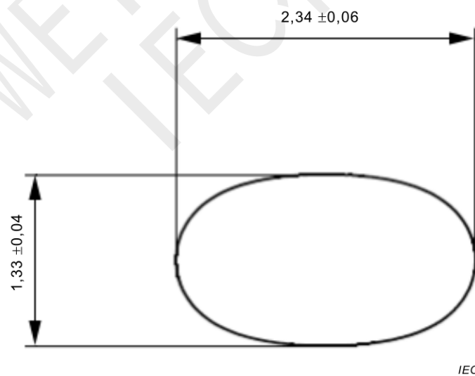
Figure D.6 – Fan jet nozzle resulting dimensions of spraying hole for checking purpose
