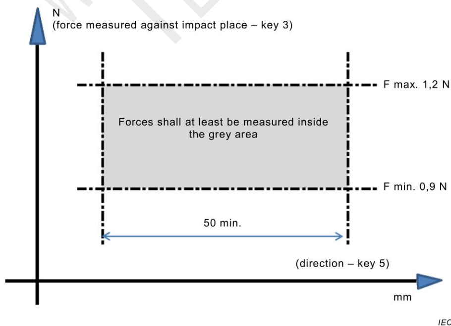
Figure D.9 – Impact force distribution
