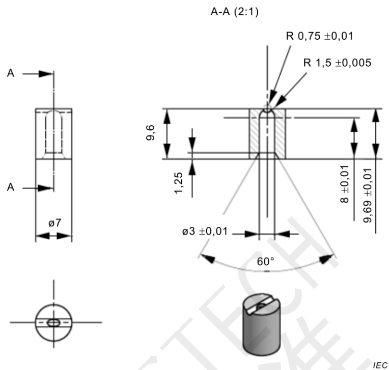
Figure D.5 – Standard test nozzle for the fan jet method
