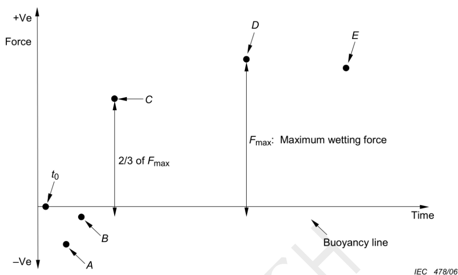
Figure 2 – Wetting conditions
