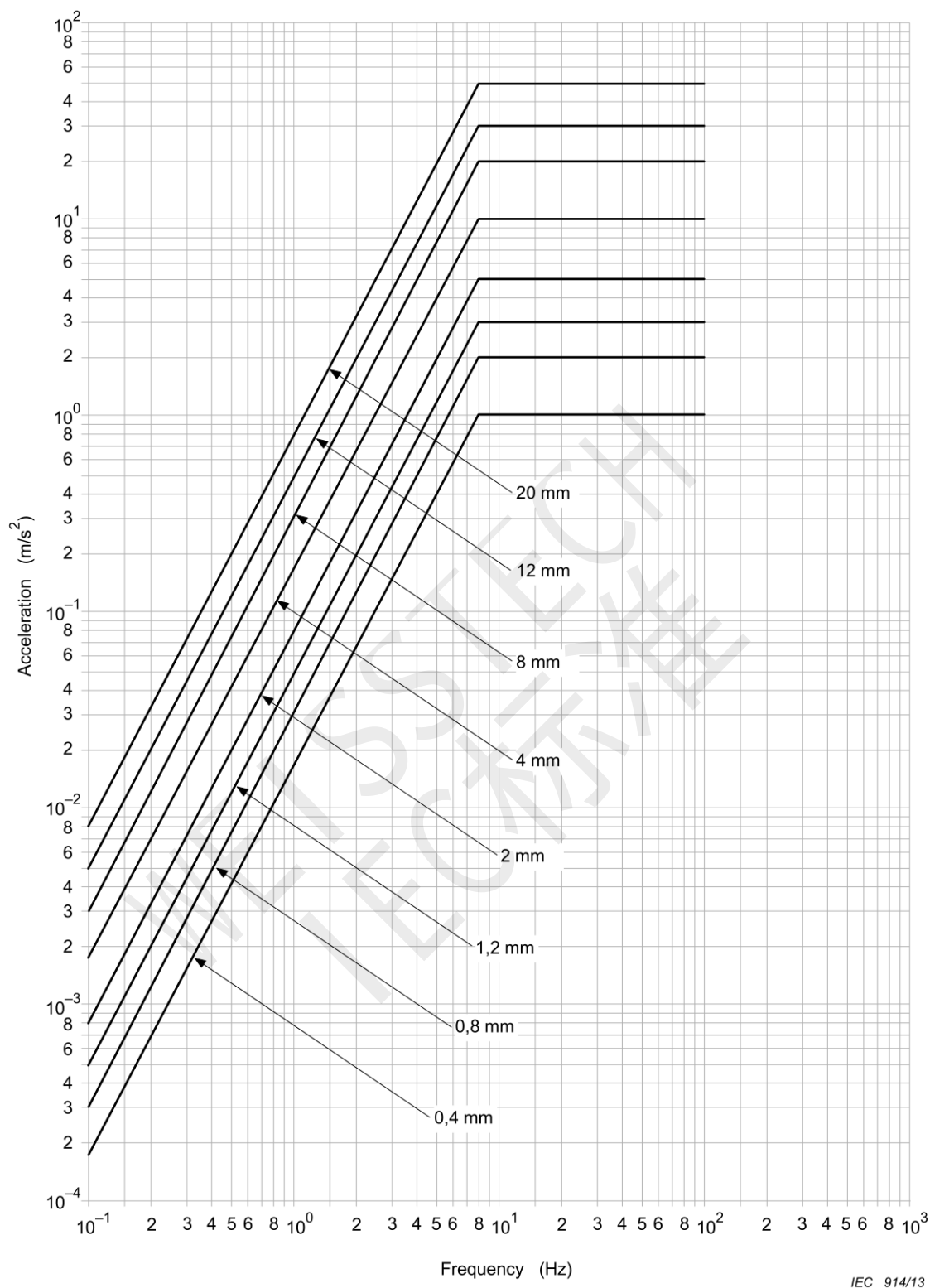
Figure 8 – Recommended test level with crossover frequency at 8 Hz
