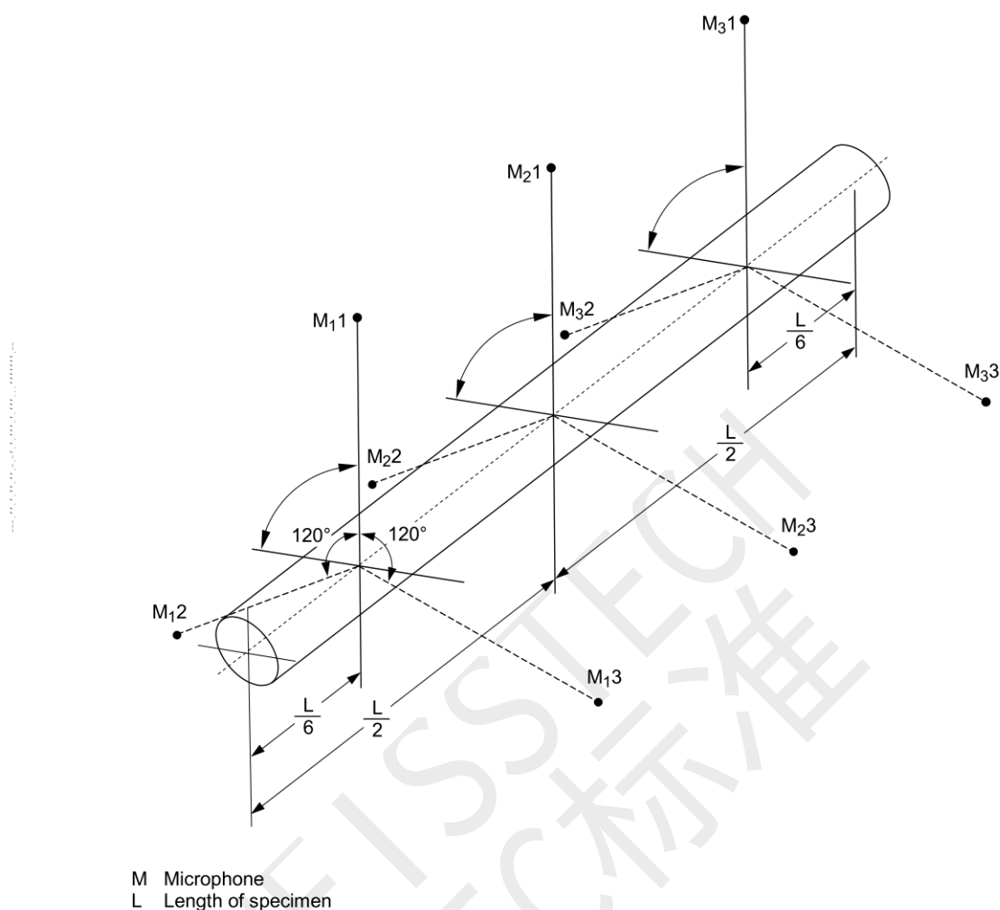
Figure A.2 – Typical microphone checkpoint arrangement around a long cylindrical specimen
