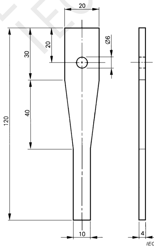
Figure B.3 – Steel spring of pendulum "c"
