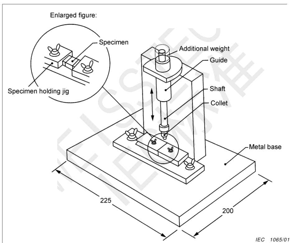
Figure 4 – Principle of test equipment
