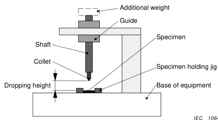
Figure 4 – Principle of test equipment
