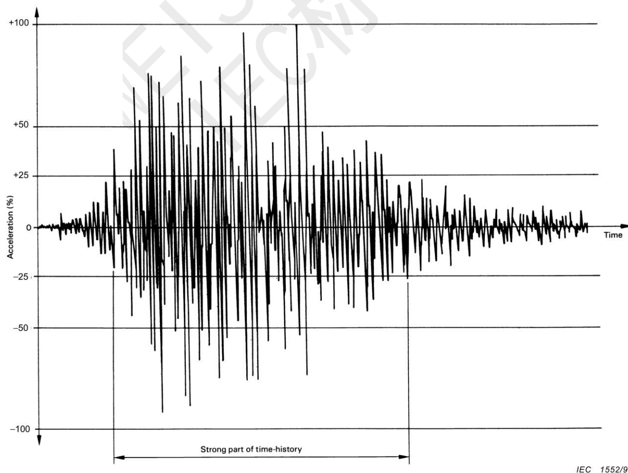
Figure 4 – Typical time-history
