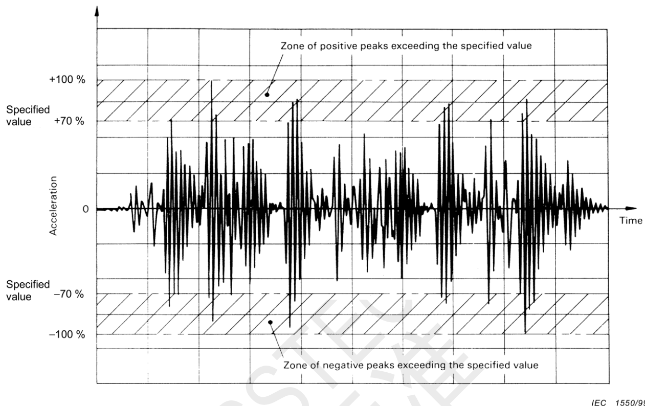
Figure 1 – Example of a typical response of an oscillator excited by a specific time-history (specified threshold value of 70 %)
