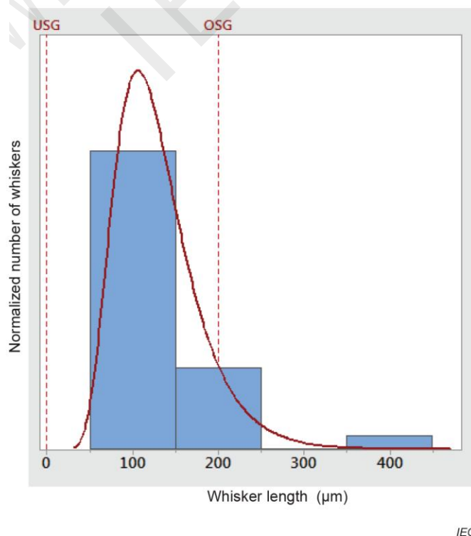
Figure C.4 – Histogram of whisker lengths and fitted log-normal distribution
