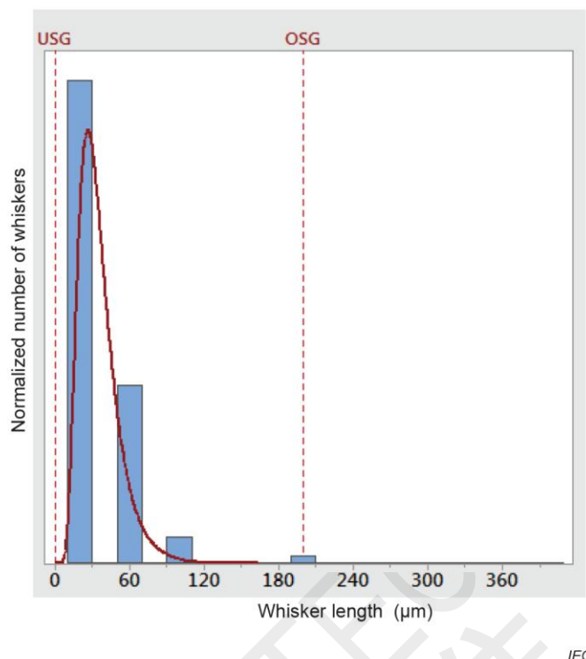
Figure C.3 – Histogram of whisker lengths and fitted log-normal distribution
