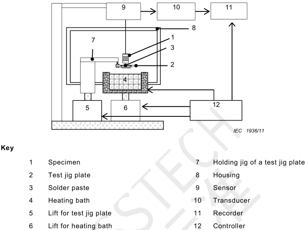
Figure 1 – Examples of the quick heating method test equipment
